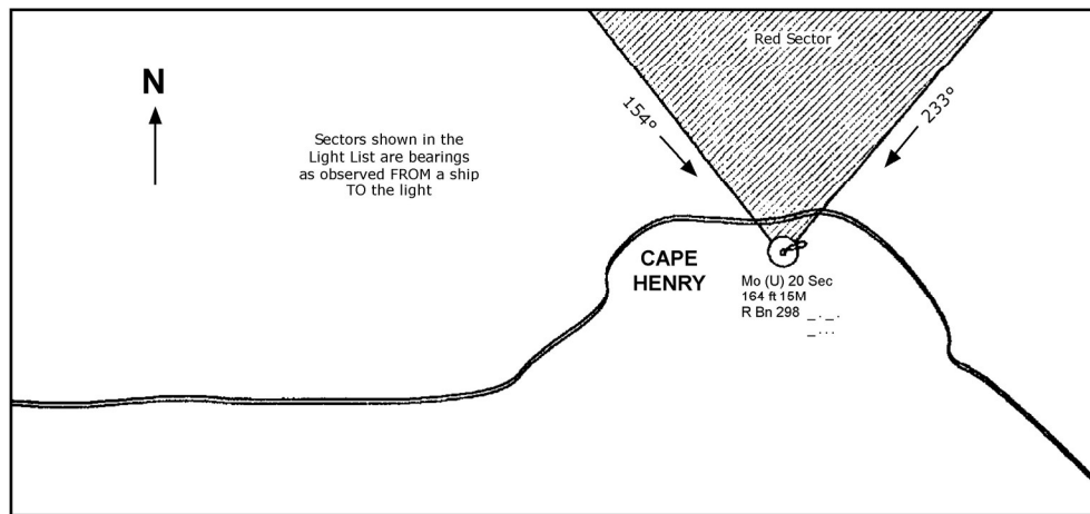
Figure 2-7 Sector Light
