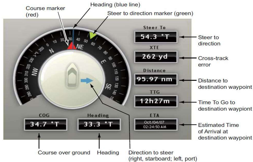
Figure 3-27 Navigation Data
