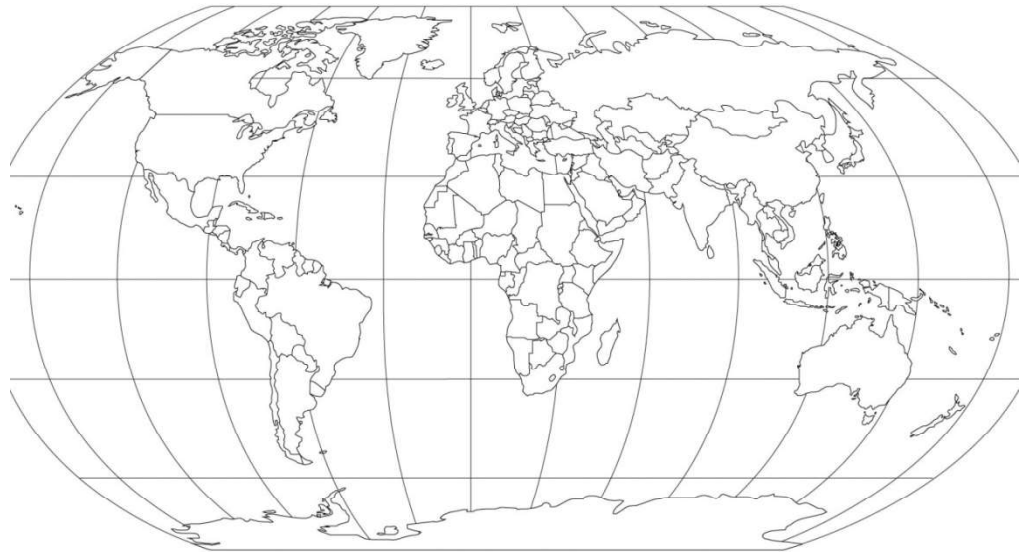
Figure 3-1 Earth with Reference Lines
